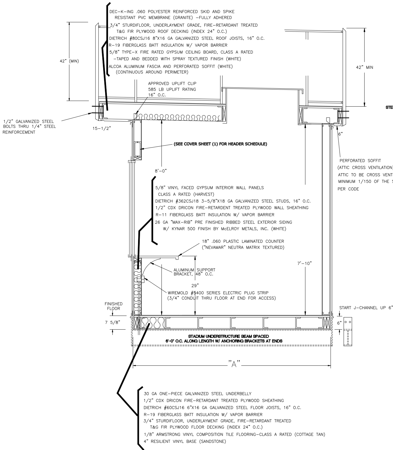
FLOOR/UNDERSTRUCTURE CONNECTION DETAIL FIELD WORK
