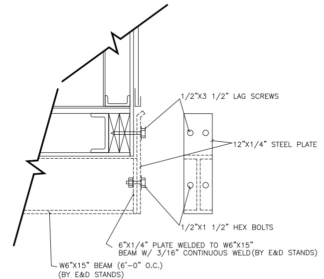
FLOOR/UNDERSTRUCTURE CONNECTION DETAIL FIELD WORK
